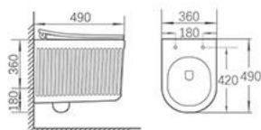
GX-4184W Rimless Wall-hung Toilet Size:490x360x360mm P-trap,180mm Roughing-in
