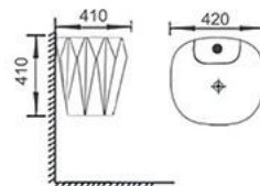
GX-7061W Wall-hung basin Size:420x410x410mm Fixing to wall with back
