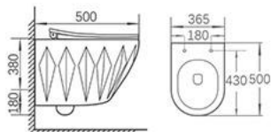
GX-4183W Rimless Wall-hung Toilet Size:500x365x380mm P-trap,180mm Roughing-in
