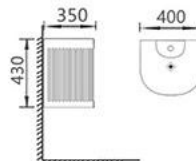
GX-7084W Wall-hung basin Size:400x350x430mm Fixing to wall with back
