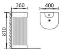
GX-7184L Pedestal basin Size:400x360x810mm Fixing to wall with back
